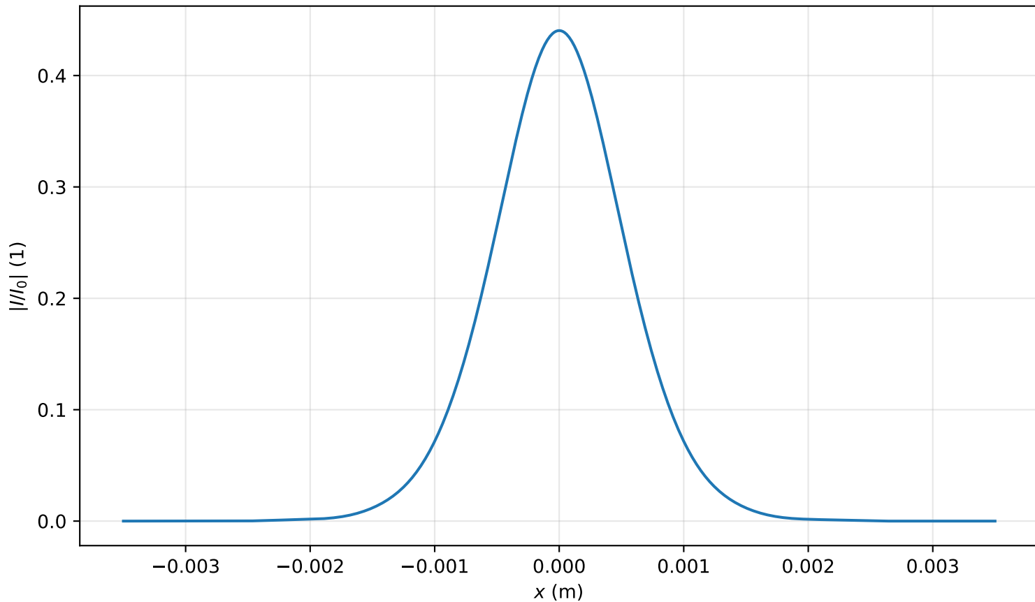
Intensity profile I(x, y = 0, z = 3.662m)/I_0 , P_{in}=0.5P_{cr} , artificial time
